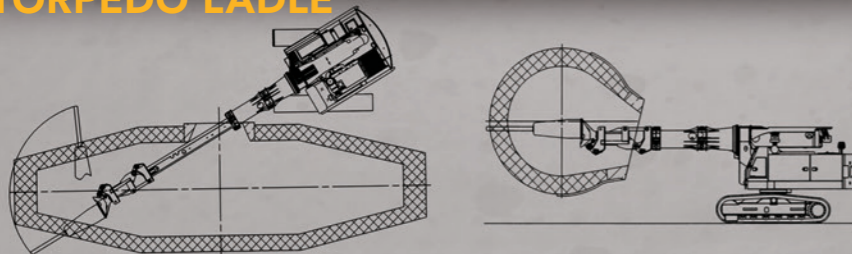
Hot Metal Transfer Car Cleanout
