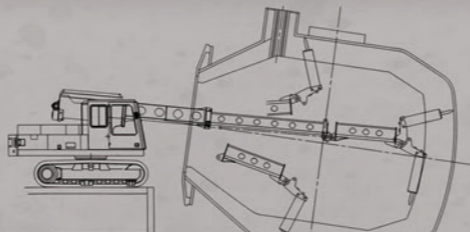
BOF Furnace Maintenance
